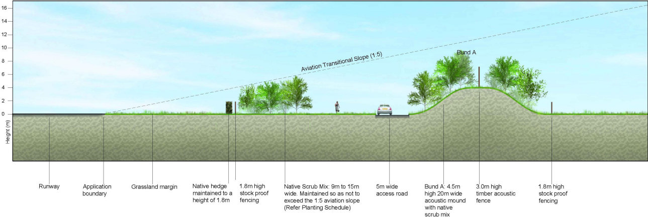
Typical Section Through Western Boundary
